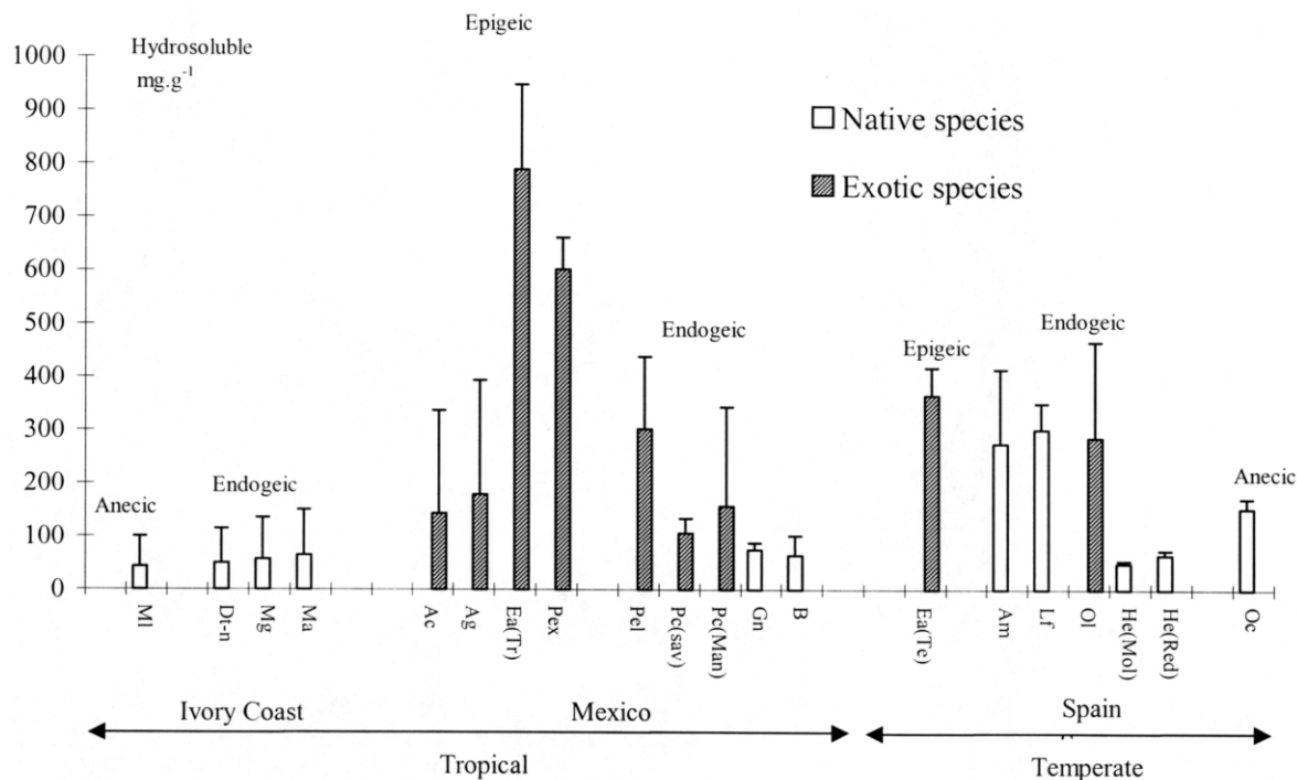
Figure 6. Anterior intestinal mucus content ( \text{mg hydro-soluble fraction} \cdot \text{g}^{-1} gut content dry weight) of earthworm species from tropical and temperate regions and of different ecological categories (epigeic, anecic and endogeic). In Ivory Coast, Millsonia lamtoiana (MI) [99], Dichogaster terrae-nigrae (Dt-n), M. ghanensis (Mg) and M. anomala (Ma) from savannahs at Lamto (Ivory Coast) [117]. In Mexico, Amyntas corticis (Ac), A. gracilis (Ag) [8], Perionyx excavatus (Pex) and Eisenia andrei in coffee pulp (Ea(Tr)); Polypheretima elongata (Pe), Glossoscolecidae sp. (Gn) and Balanteodrilus sp. (B) in a savannah-pasture Alfisol and Pontoscolex corethrurus under pastures in an Alfisol (Pc(sav)) and Entisol (Pc(Man)) [168]. In Spain, E. andrei in cow manure (Ea(Te)), Hormogaster elisae from pasture soil at El Molar (He(Mol)) and woodland soil at Redueña (He(Red)); Lumbricus friendi (Lf), Octodrilus complanatus (Oc) [168], Allolobophora molleri (Am) [166] and Octolasion lacteum (OI) [167].
