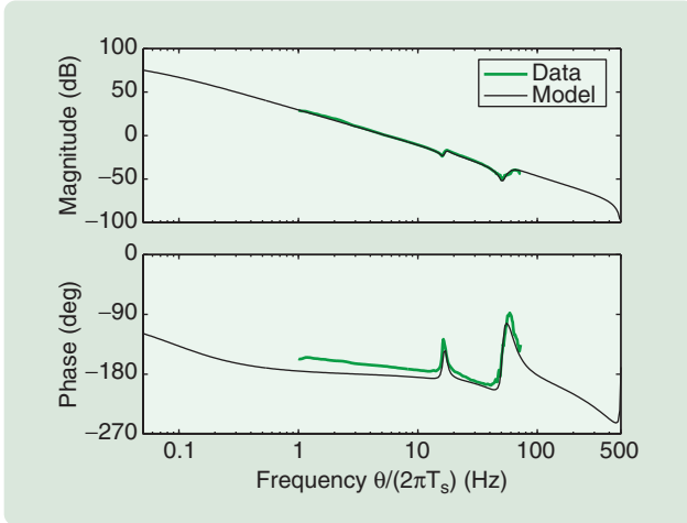
FIGURE 6 Experimental frequency response and model of the \mu -RD x axis with sampling period T_s = 0.001 s. The experimental data are obtained from 1–70 Hz. Outside this range nonlinearities appear in the form of static friction at low frequencies and high signal-to-noise ratio at high frequencies. The frequency response shows dominant double-integrator dynamics with structural resonances at 16 Hz and 55 Hz.
