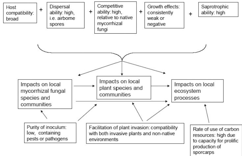
Figure 1 A conceptual model illustrating issues of primary concern when using fungal inoculum in plant management. The top row represents traits of non-native mycorrhizal inoculum that are hypothesized to be associated with impacts on native communities and ecosystem processes. These are often the very same traits sought after as favourable attributes for management use. The middle row represents three primary areas of potential impacts and their interactions. The bottom row represents mechanisms by which fungal inocula may either directly or indirectly affect natural systems.
