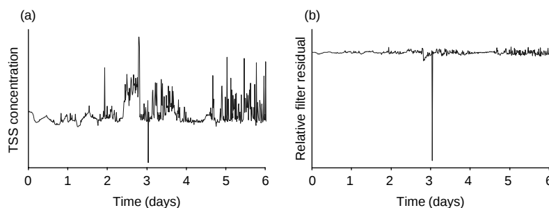
Figure 3 TSS sensor data with increasing variability (a) and the relative filter residuals for the same data (b)
